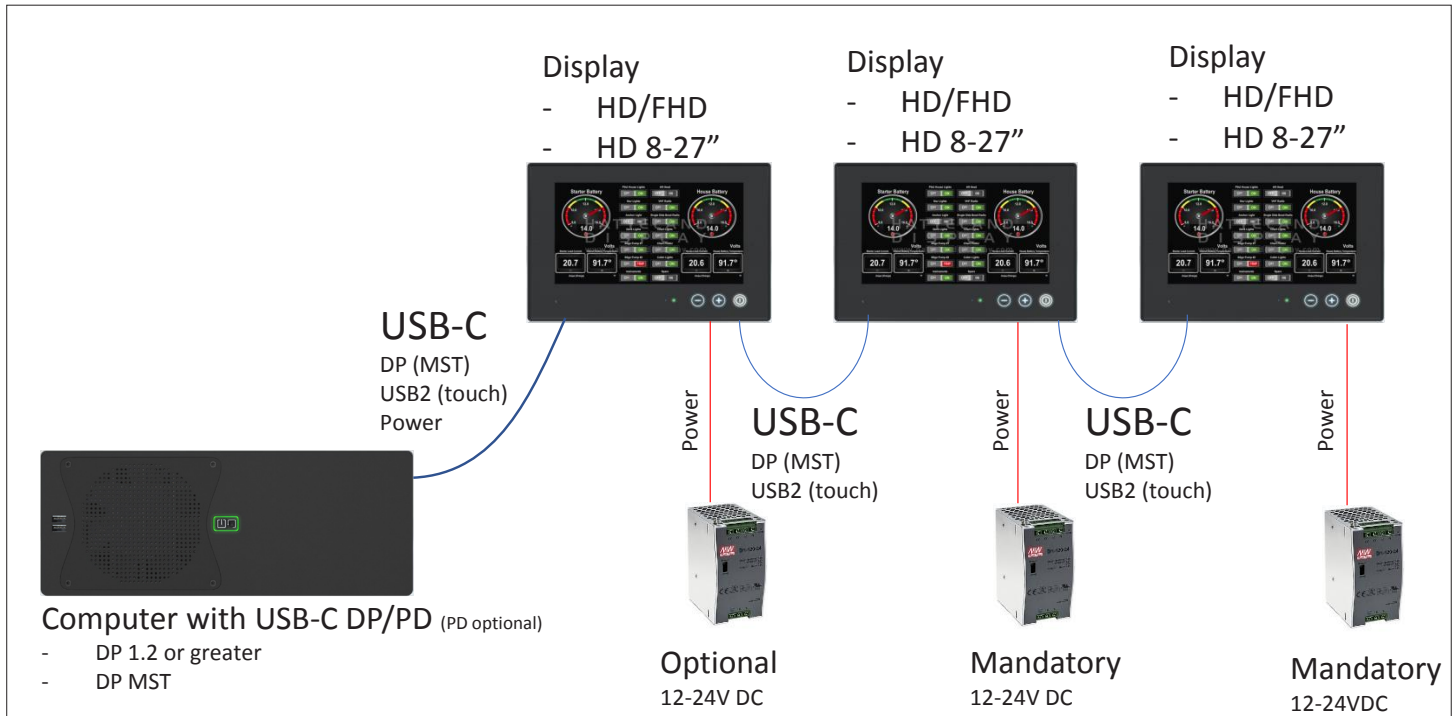
Illustration: USB-C Dasiy chaning, upto 3x FHD dispalys with touch. First display can be powered via USB-C.
