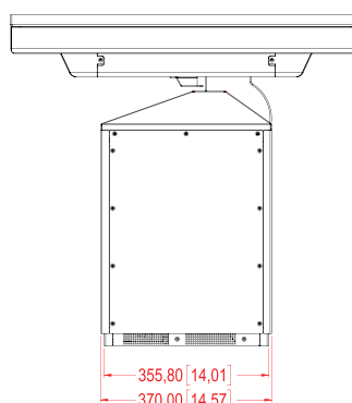
LEFT VIEW
