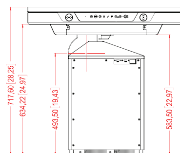
RIGHT VIEW
