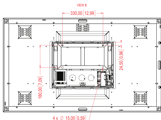
BOTTOM VIEW Floor Mounting Pattern
