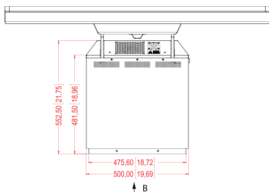
BOTTOM VIEW Floor Mounting Pattern
