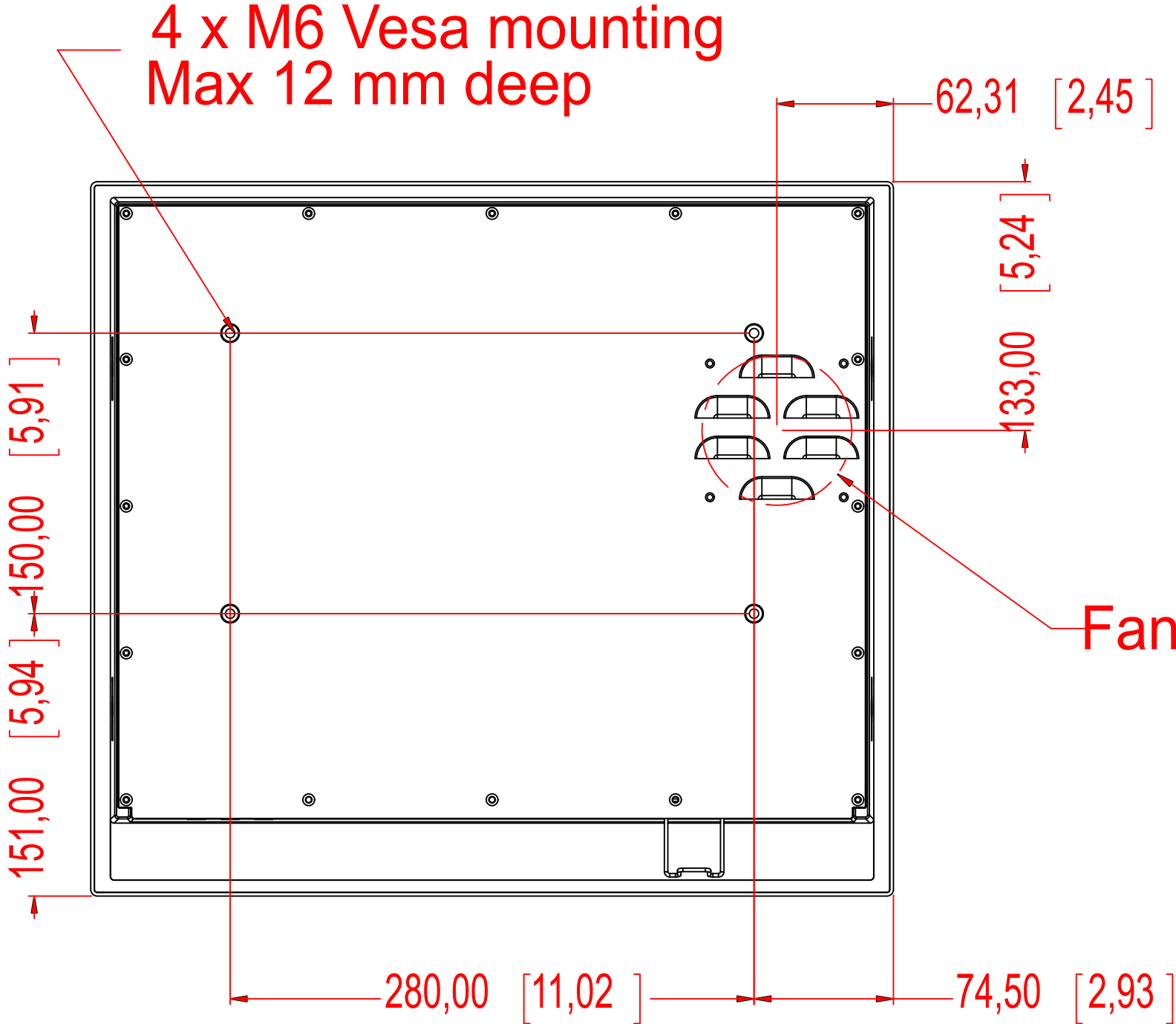
BACK VIEW
