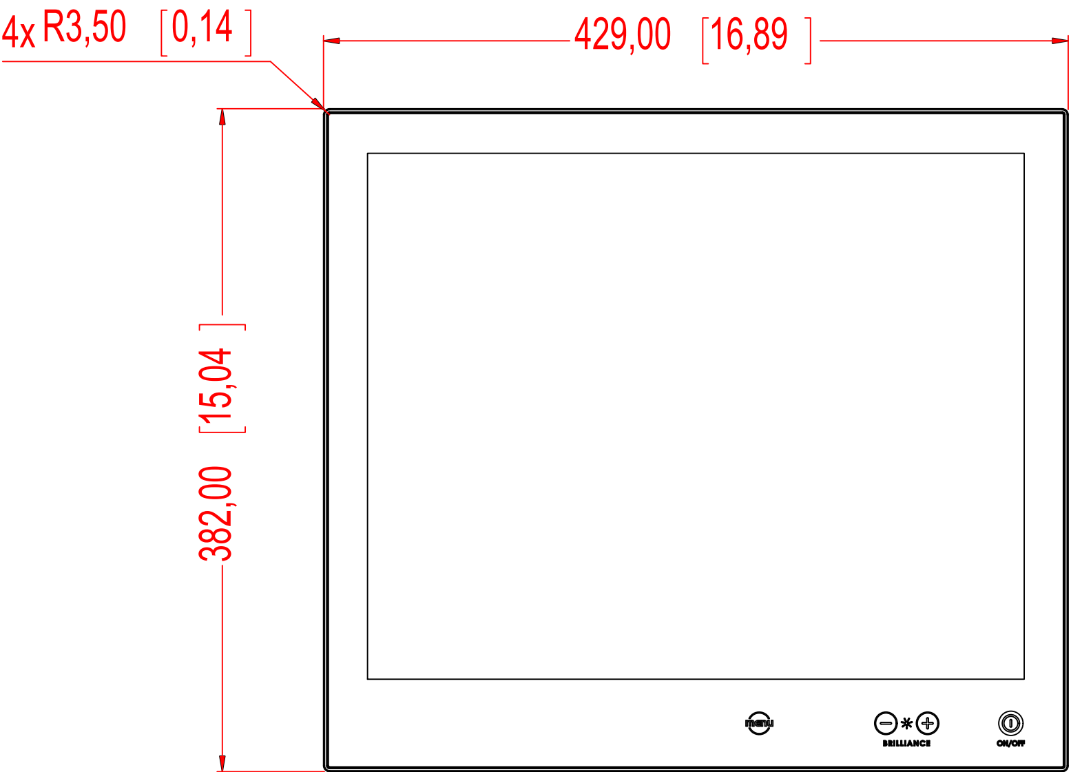
FRONT VIEW
