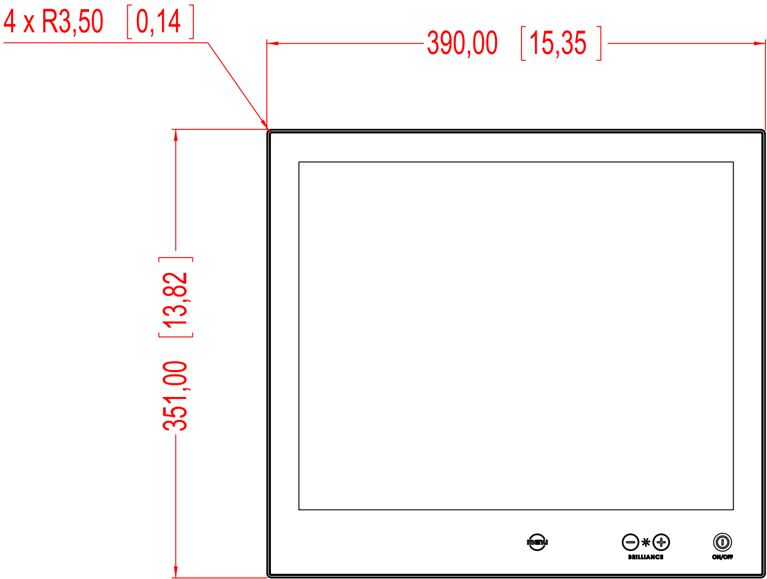
FRONT VIEW
