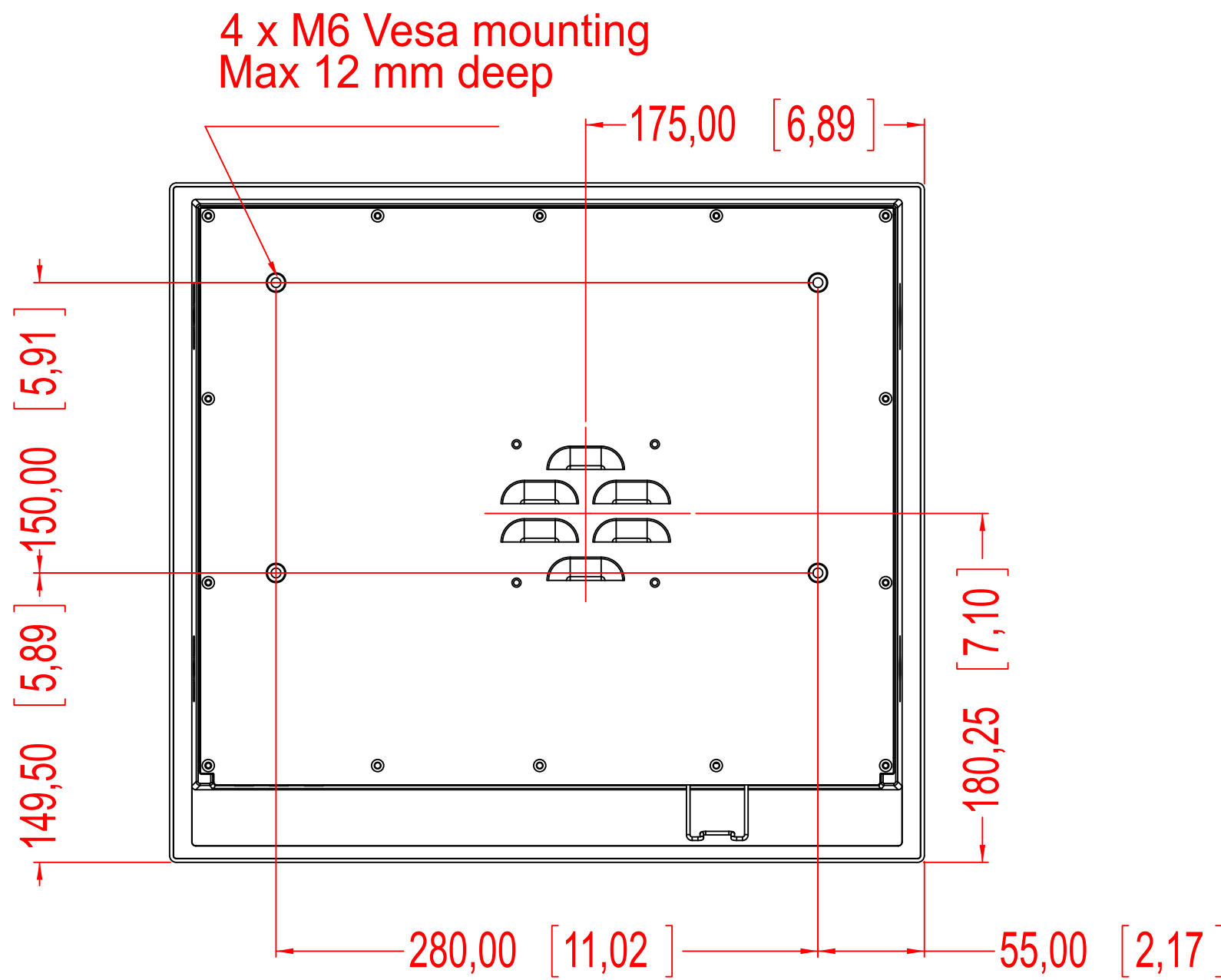
BACK VIEW
