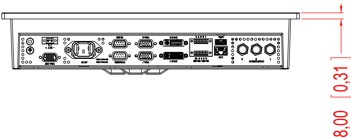
BOTTOM VIEW
