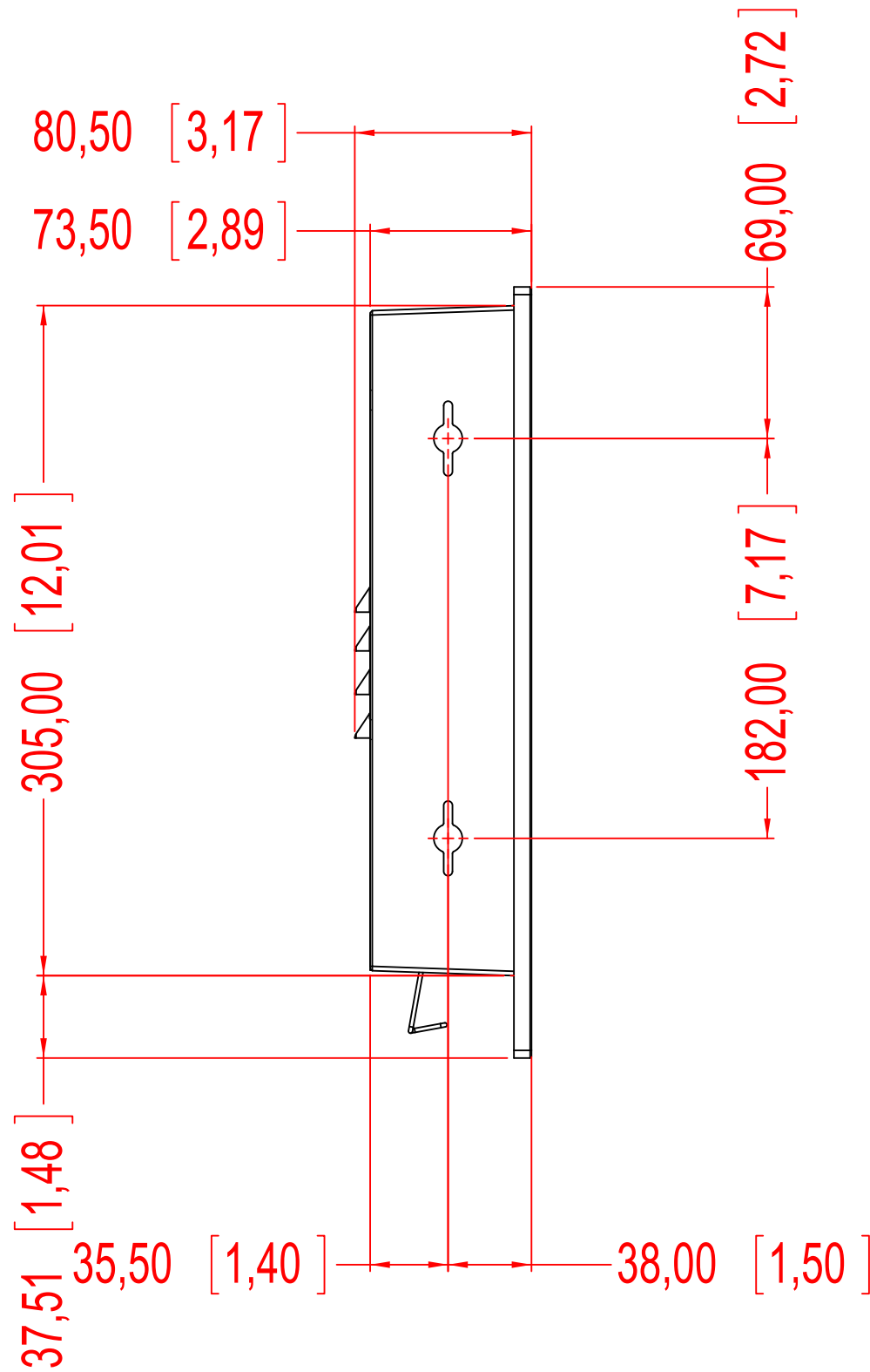
SIDE VIEW
