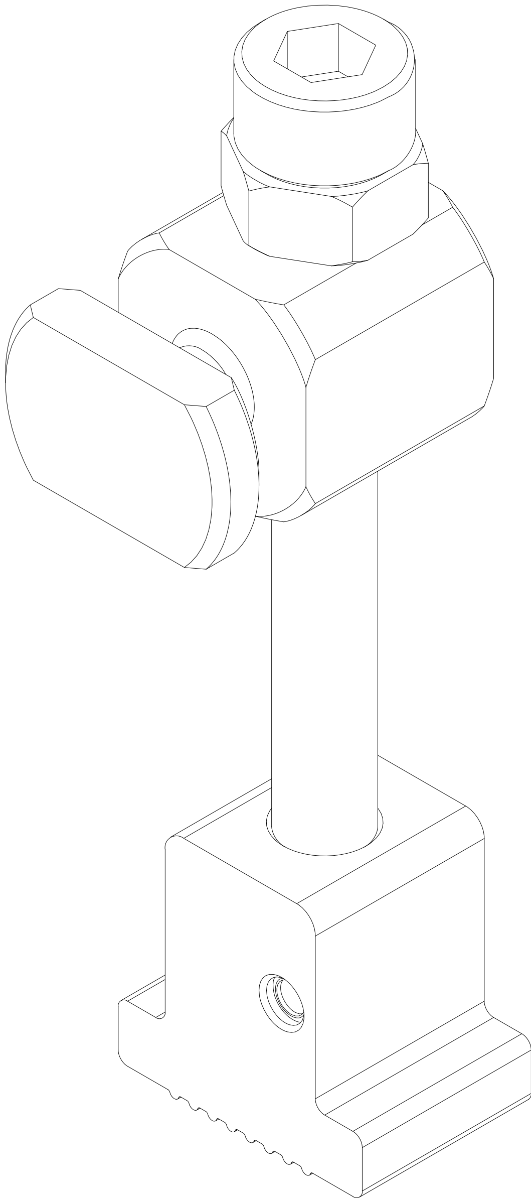
DIMETRIC VIEW
