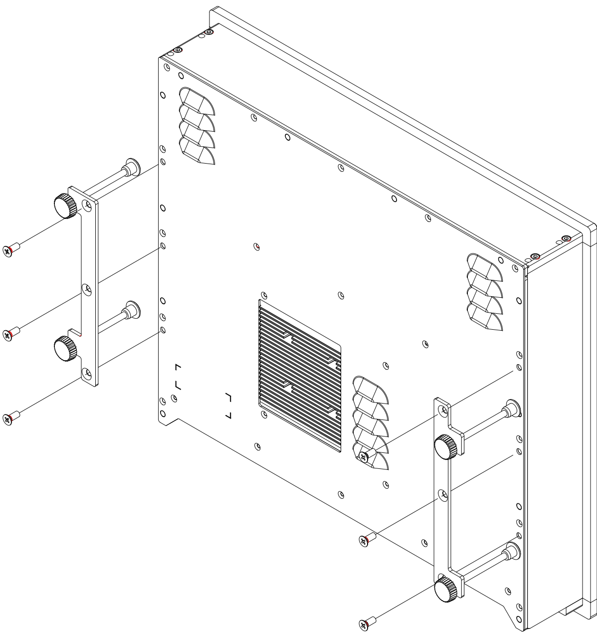
DIMETRIC VIEW
