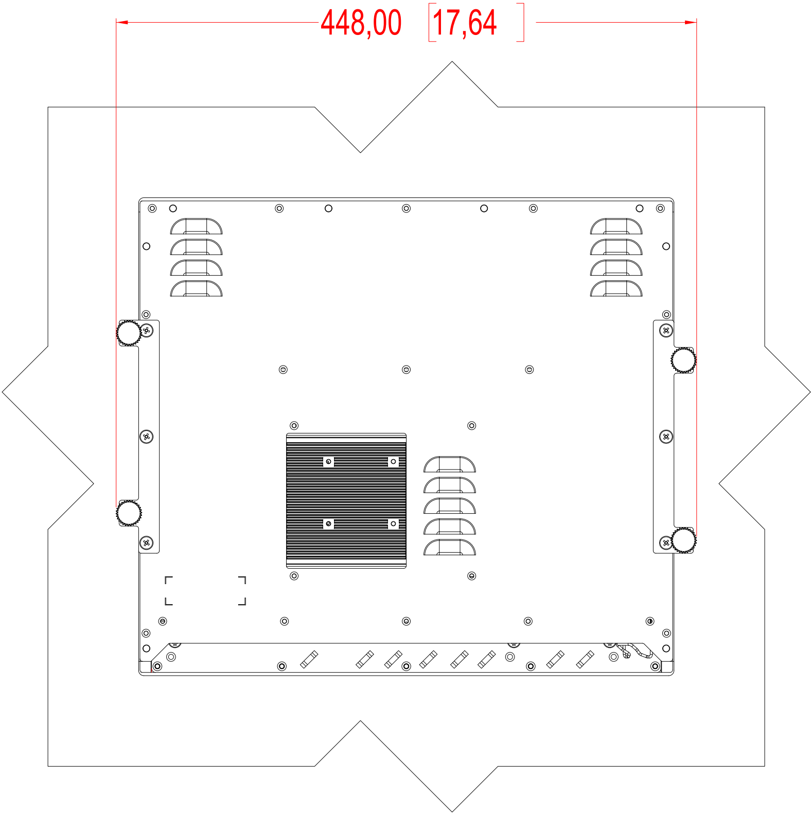
BACK VIEW
