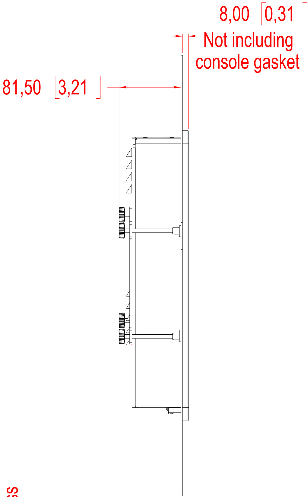
SIDE VIEW
