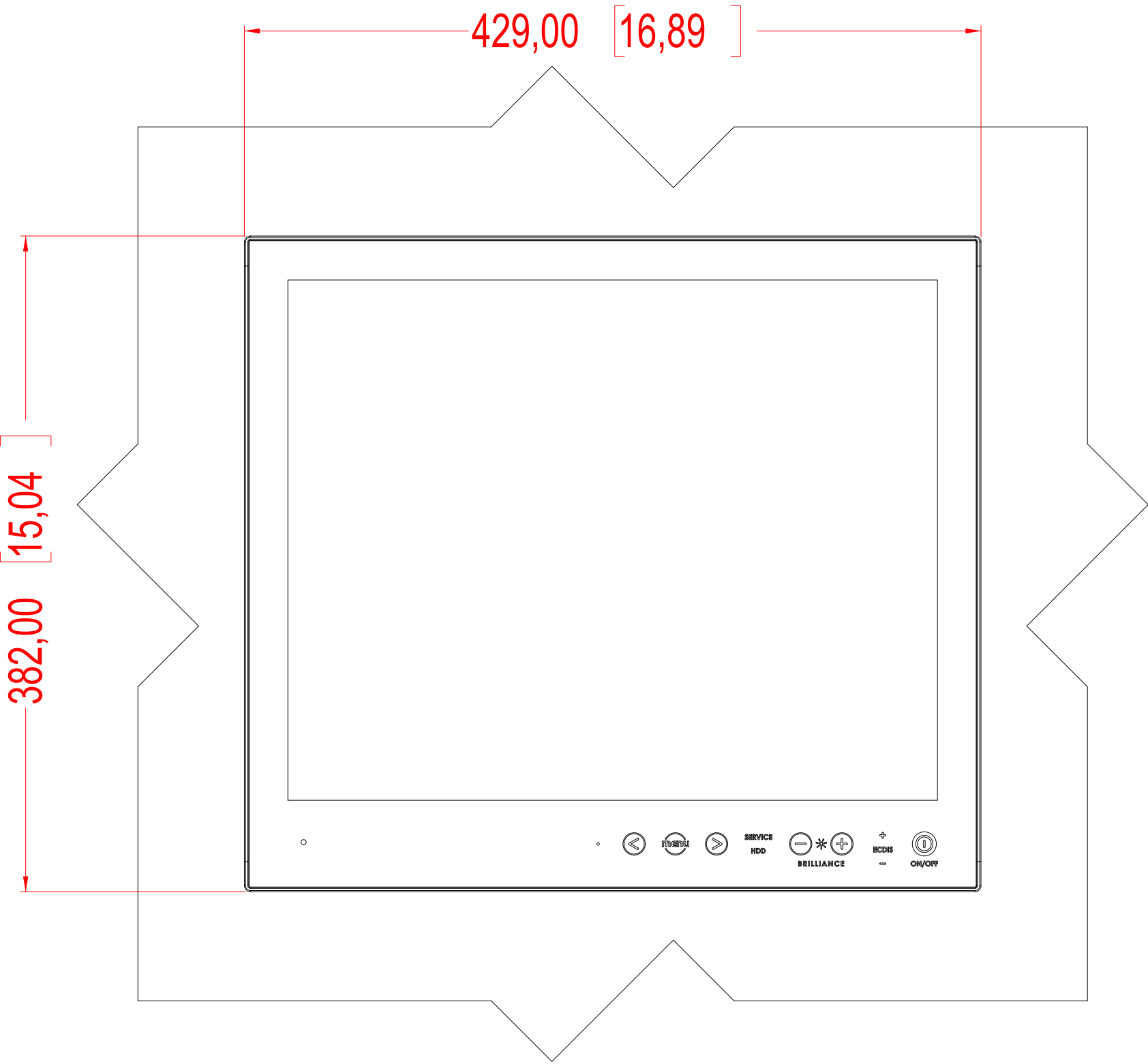
FRONT VIEW
