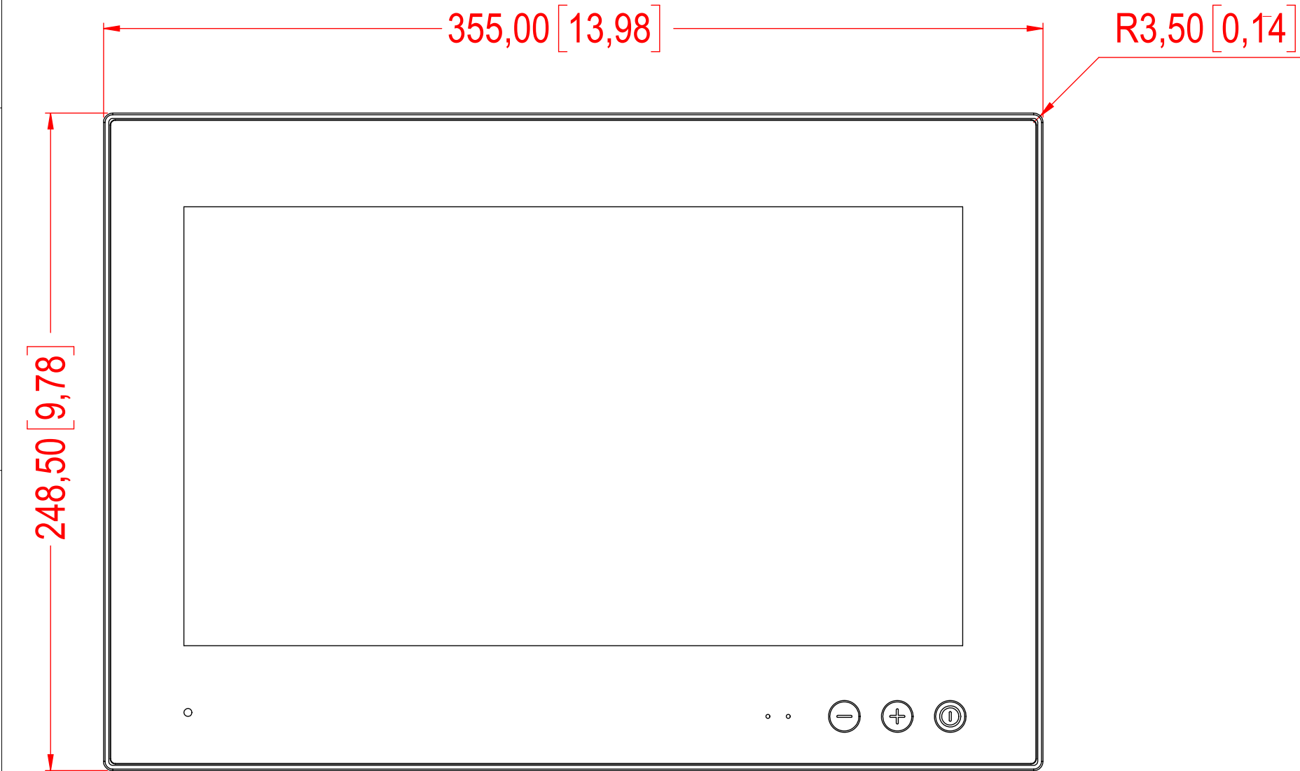
FRONT VIEW
