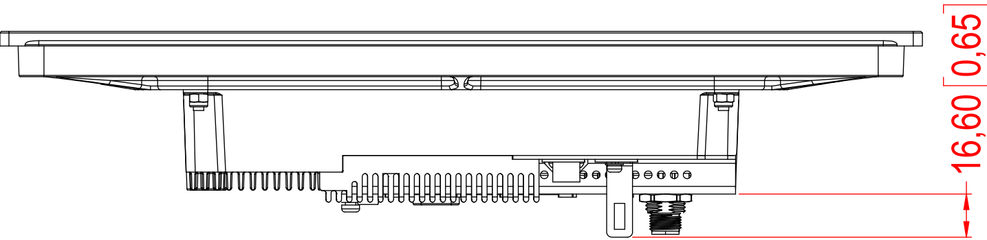
BOTTOM VIEW
