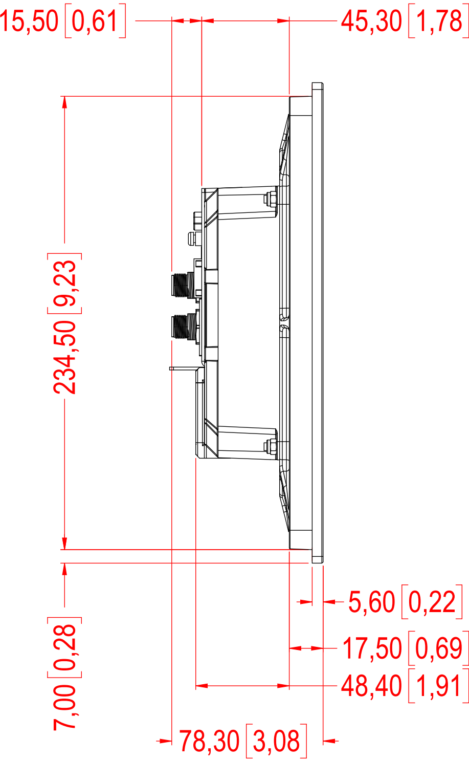
SIDE VIEW
