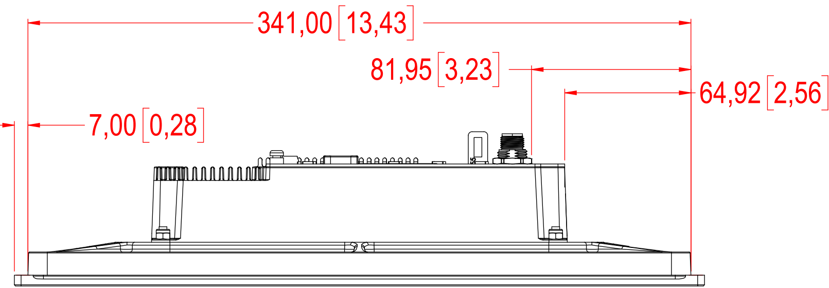
TOP VIEW
