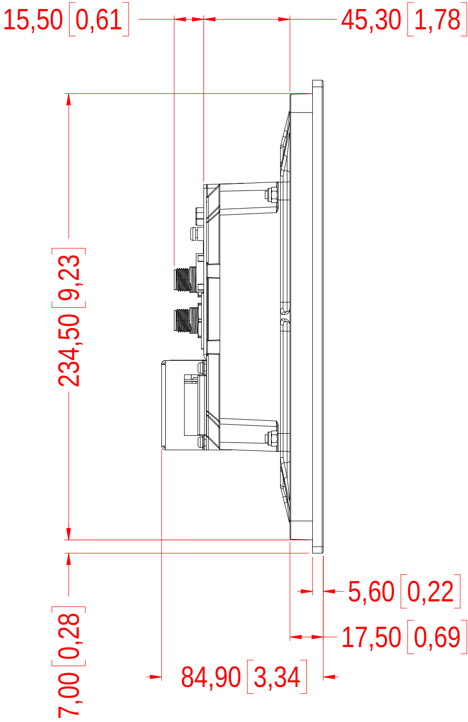
SIDE VIEW
