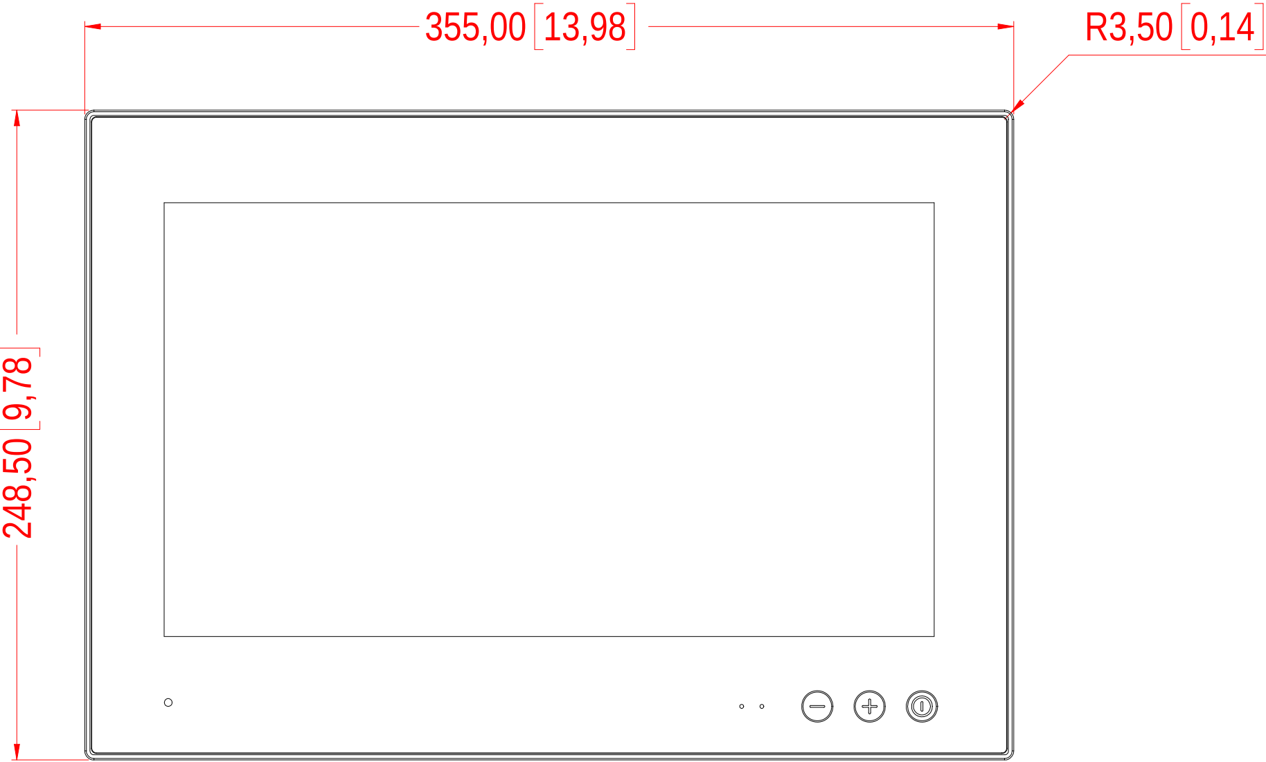
FRONT VIEW
