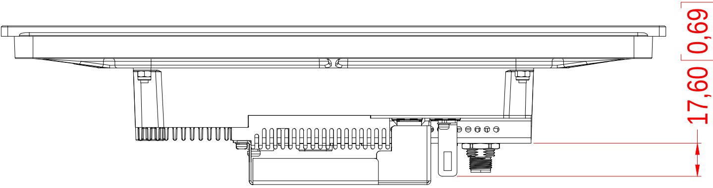
BOTTOM VIEW
