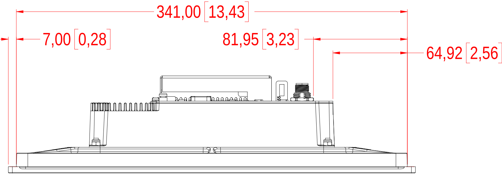
TOP VIEW
