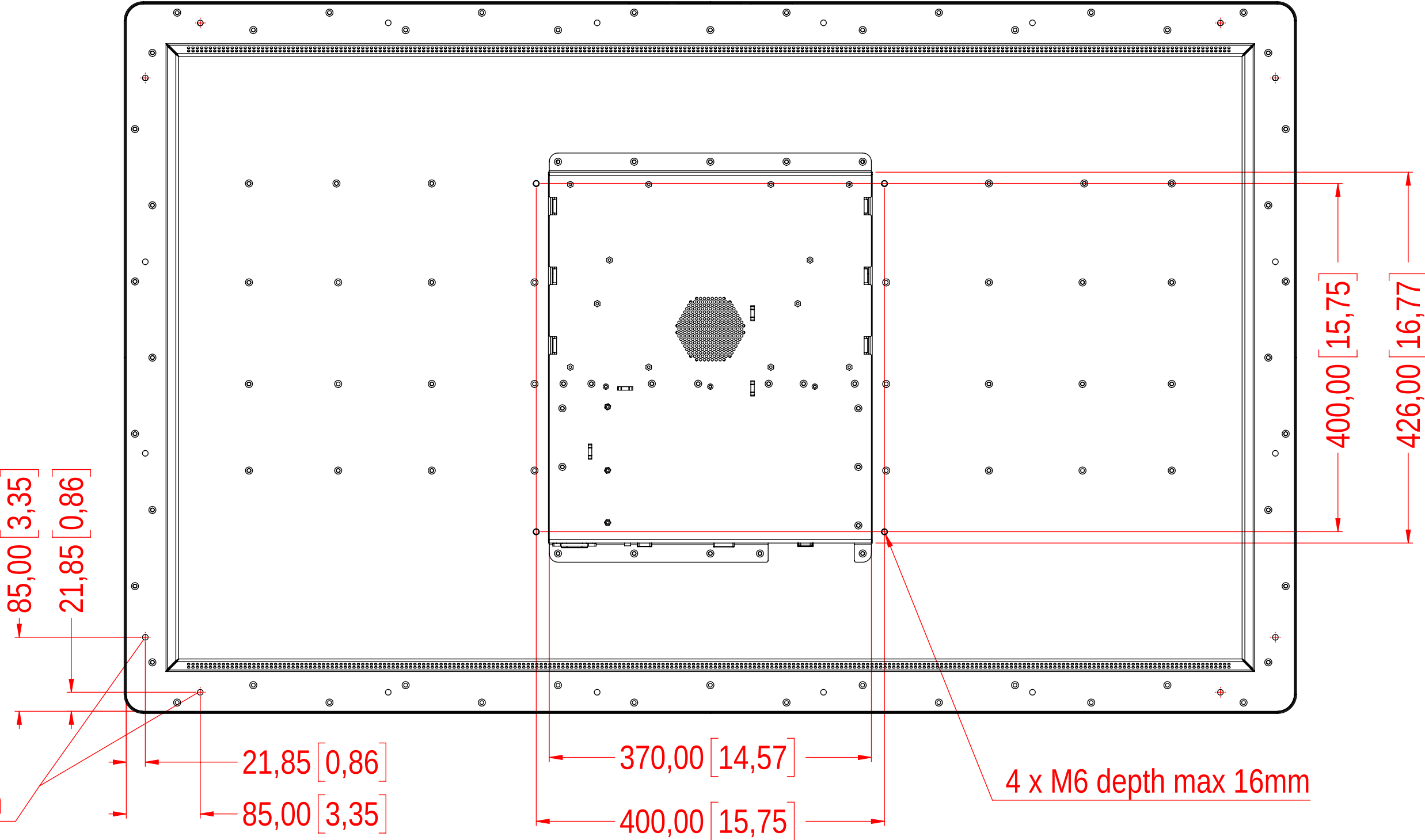
BACK VIEW
