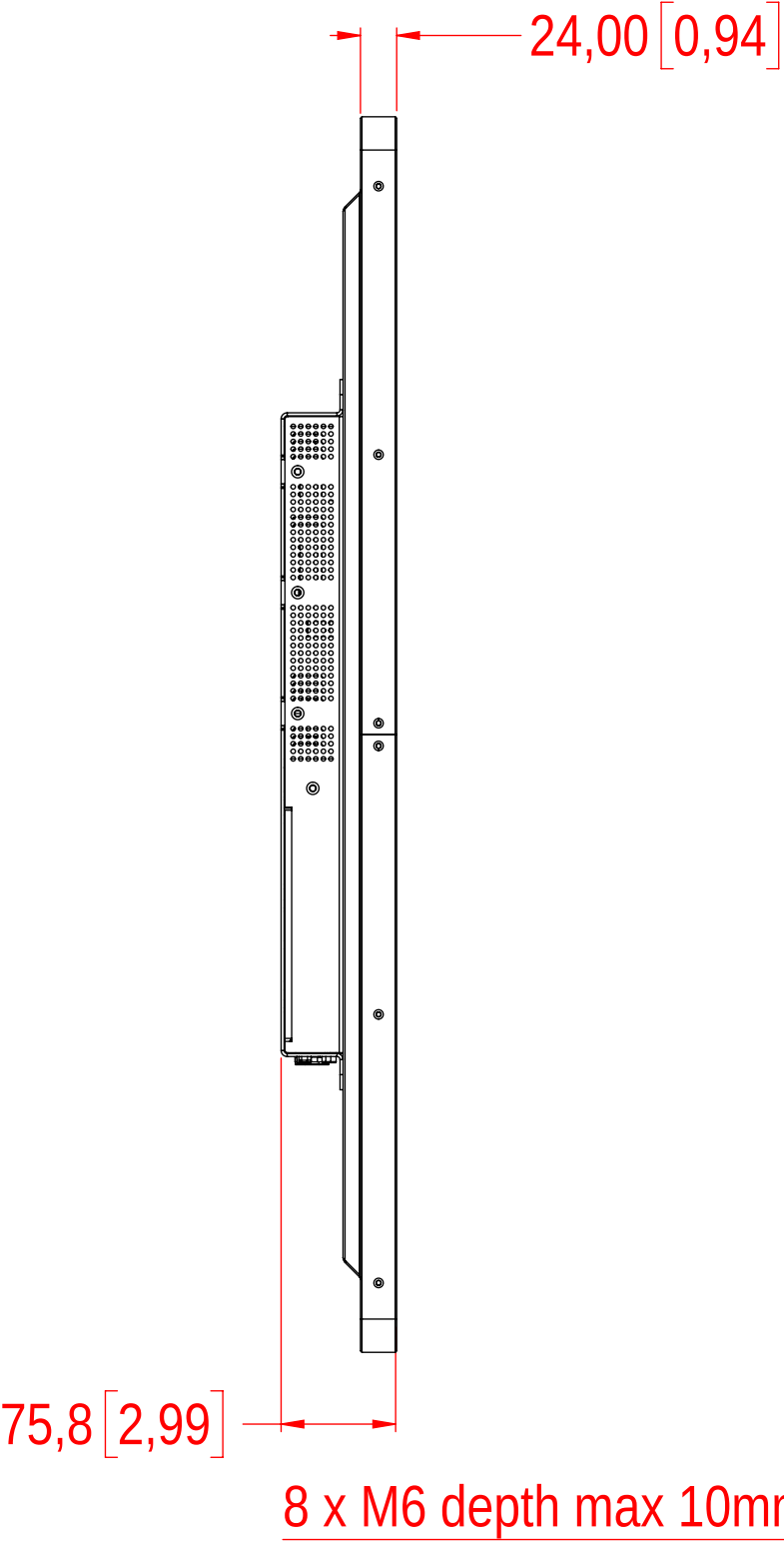
SIDE VIEW
