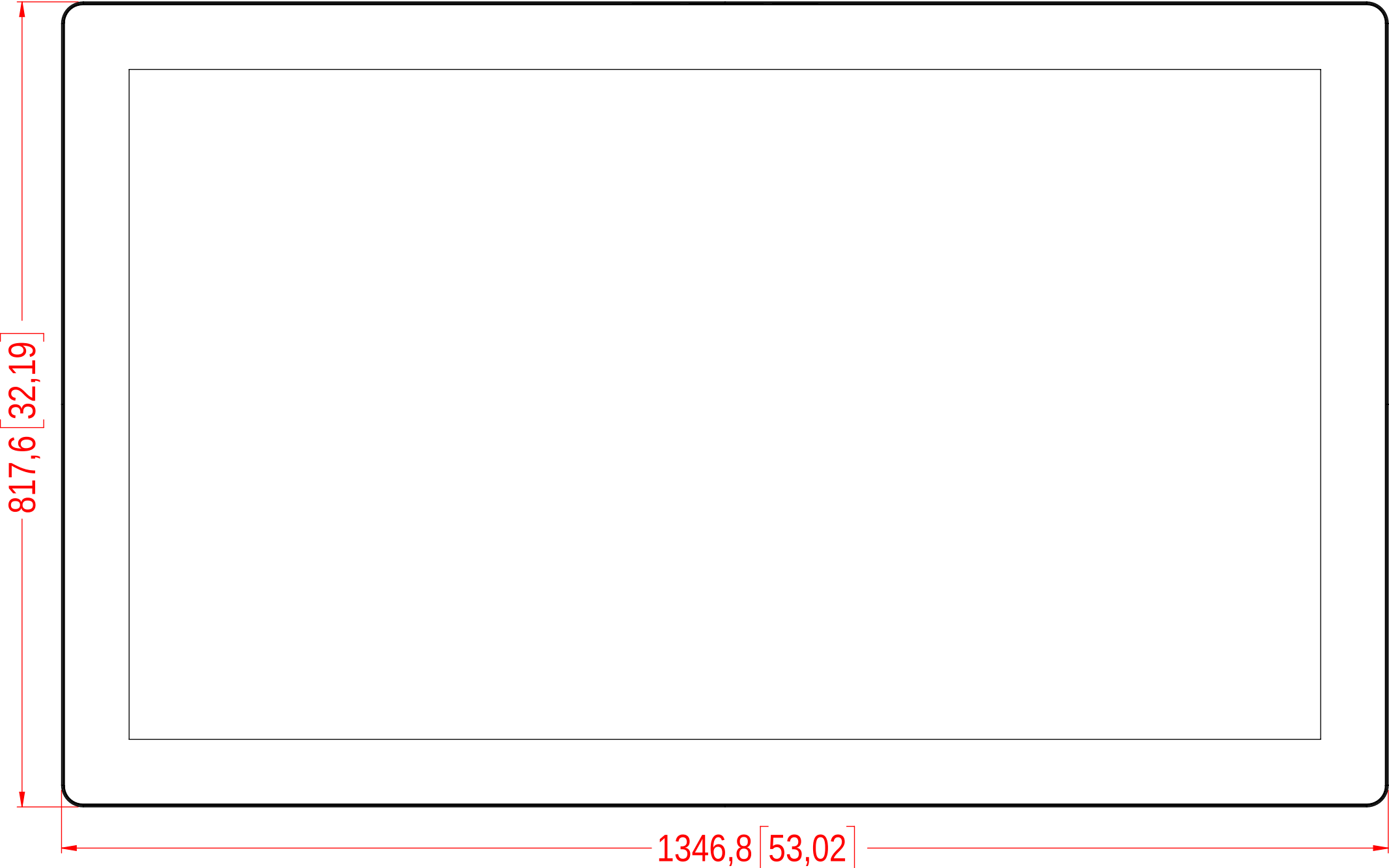
FRONT VIEW
