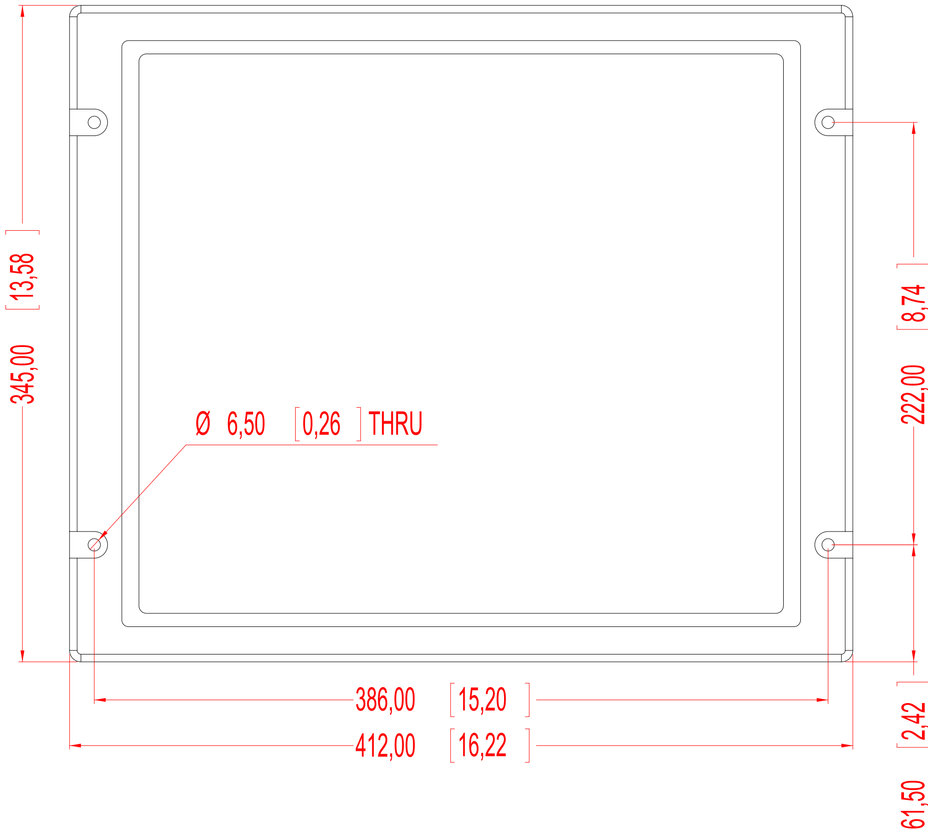
FRONT VIEW
