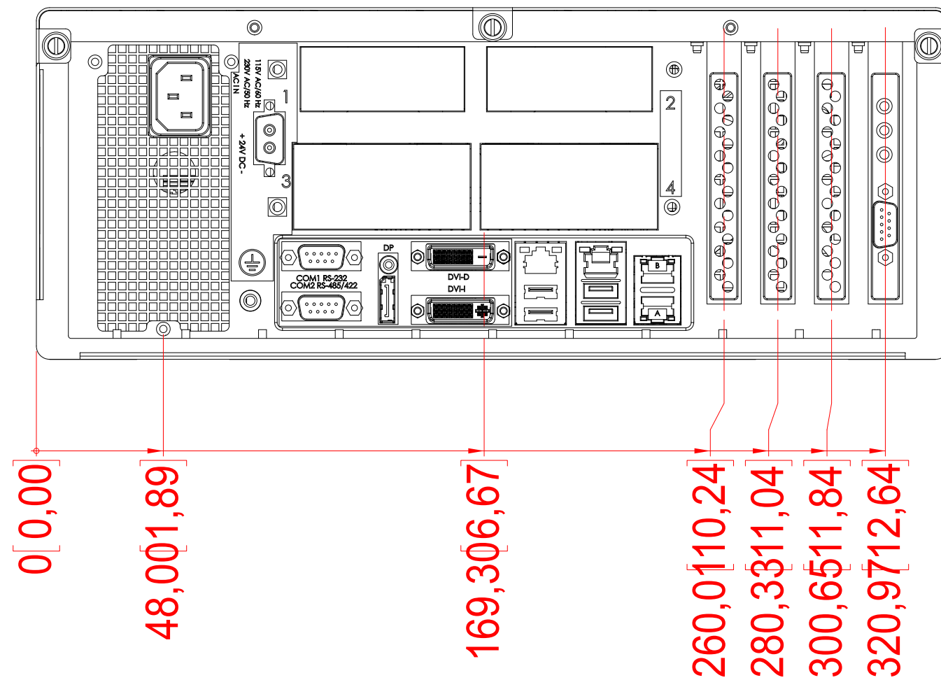
BACK VIEW
