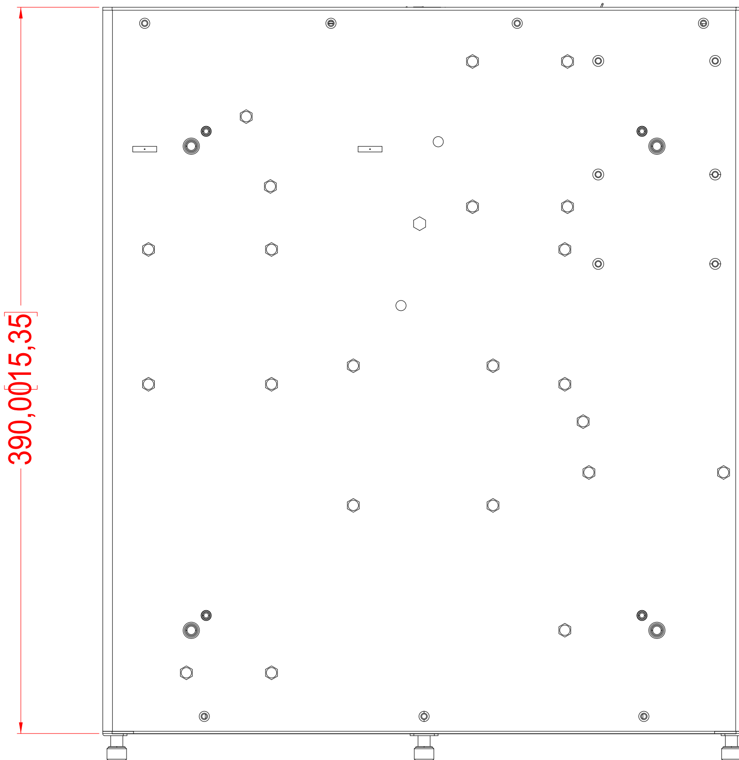
BOTTOM VIEW
