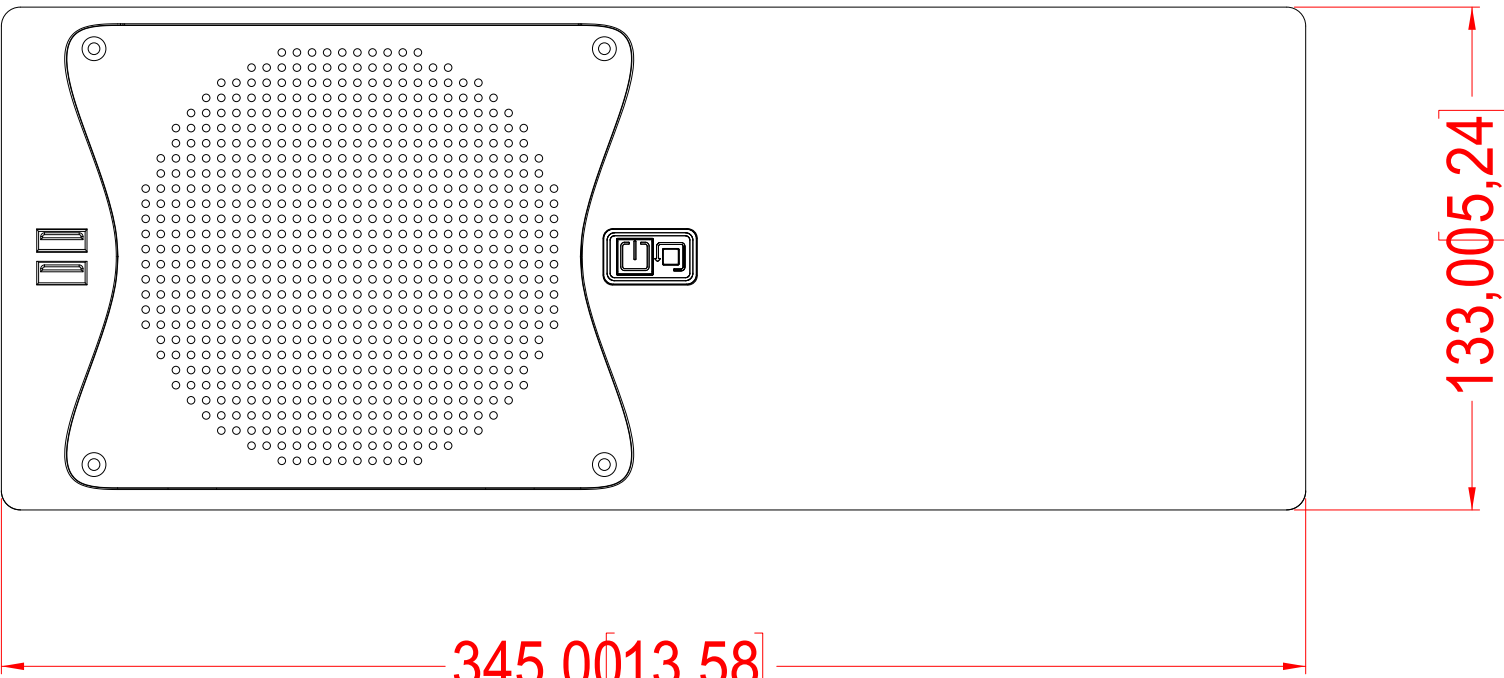
FRONT VIEW
