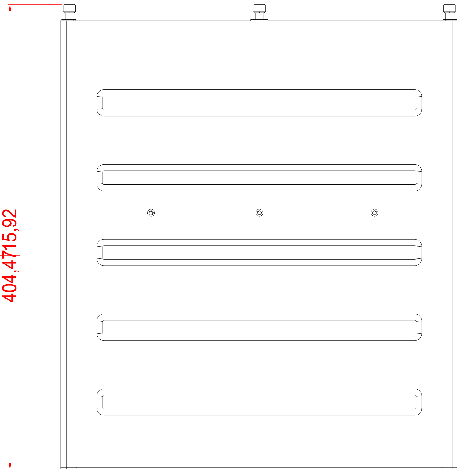
TOP VIEW
